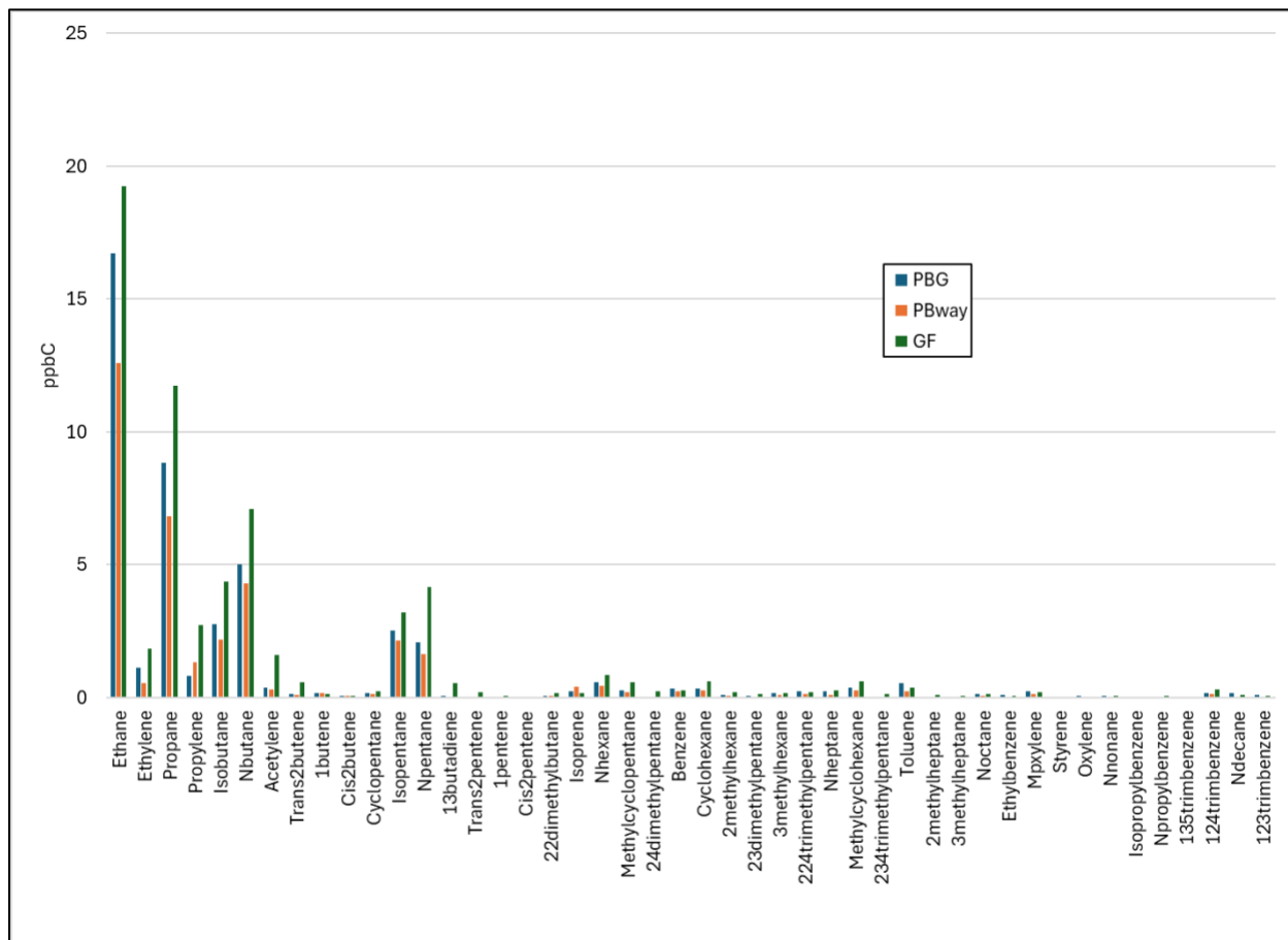
Figure 16. January 1 through October 31, 2025, mean concentrations of individual hydrocarbon species at three air monitoring stations.
