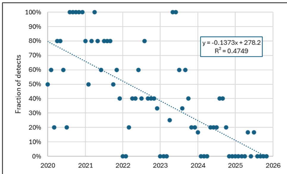
Figure 11. PBG percent of detections by sample each month, Jan. 2020 to Nov. 2025
