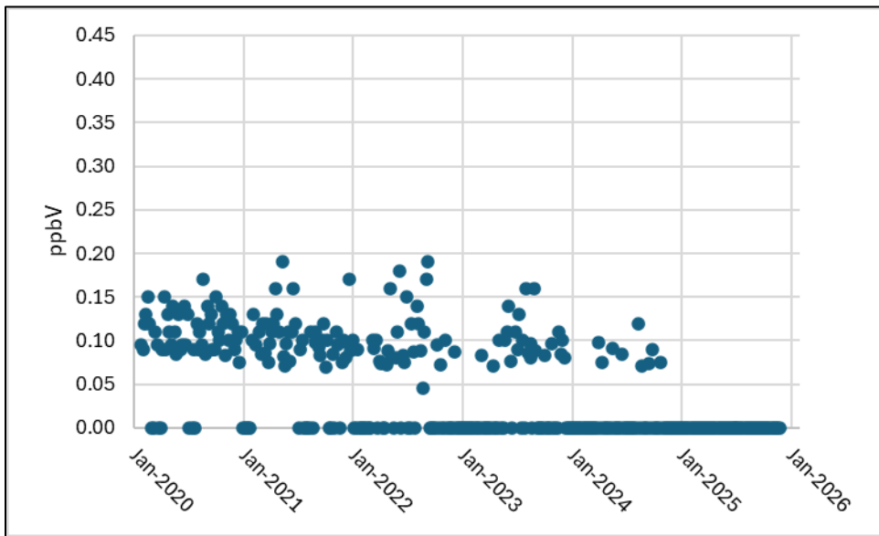
Figure 9. PBway EtO concentrations, every 6 th day samples Jan. 2020 through Nov. 2025
