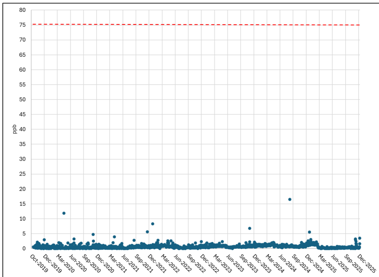
Figure 19. Daily maximum SO 2 at GF, Oct. 1, 2019 – Dec. 31, 2025, with EPA NAAQS Value 75 ppb (red dashed line).
