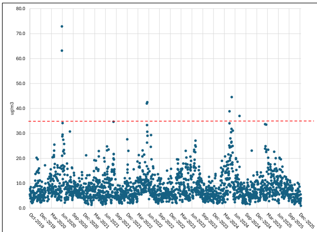
Figure 17. Averaged 24-Hour PM 2.5 at GF, Oct. 1, 2019 – Dec. 31, 2025, with EPA NAAQS Value 35 \mu\text{g}/\text{m}^3 .
