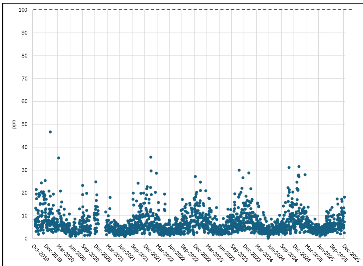
Figure 18. Daily maximum NO 2 at GF, ppb units, Oct. 1, 2019 – Dec. 31, 2025, with EPA NAAQS Value 100 ppb (red dashed line)
