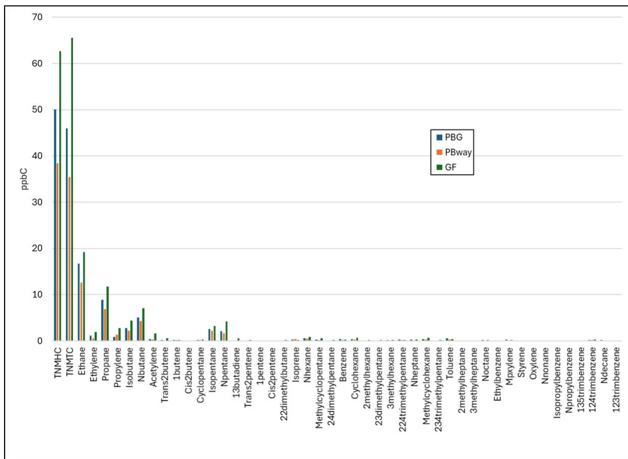
Figure 15. January 1 through Oct. 31, 2025, mean concentrations of TNMTC, TNMHC, and hydrocarbon species at three stations.
