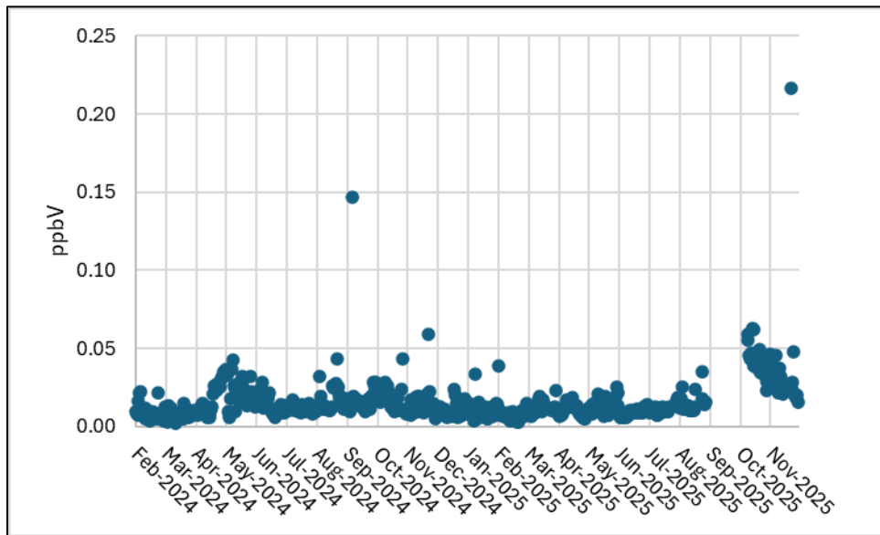
Figure 13. PBG AROMA EtO continuous analyzer 24-hour averages, Feb. 1, 2024 – Nov. 30, 2025
