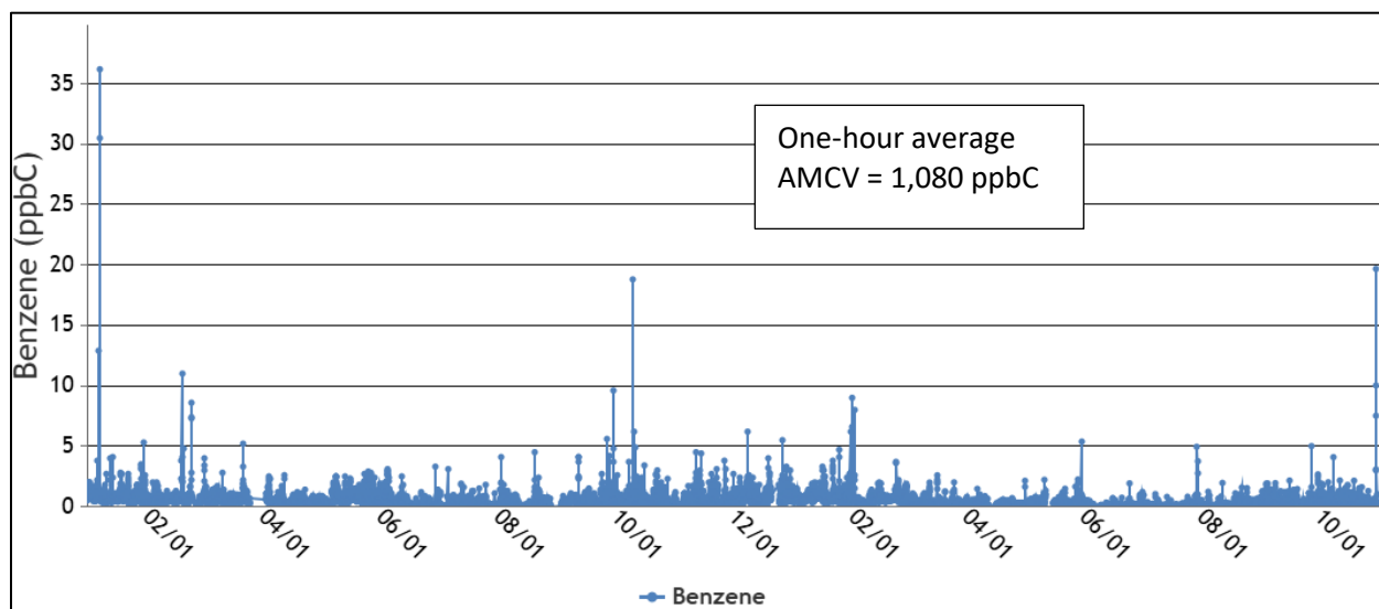
Figure 5. Hourly benzene concentrations at PBG station, Jan. 1, 2024 – Oct. 31, 2025, ppbC units
