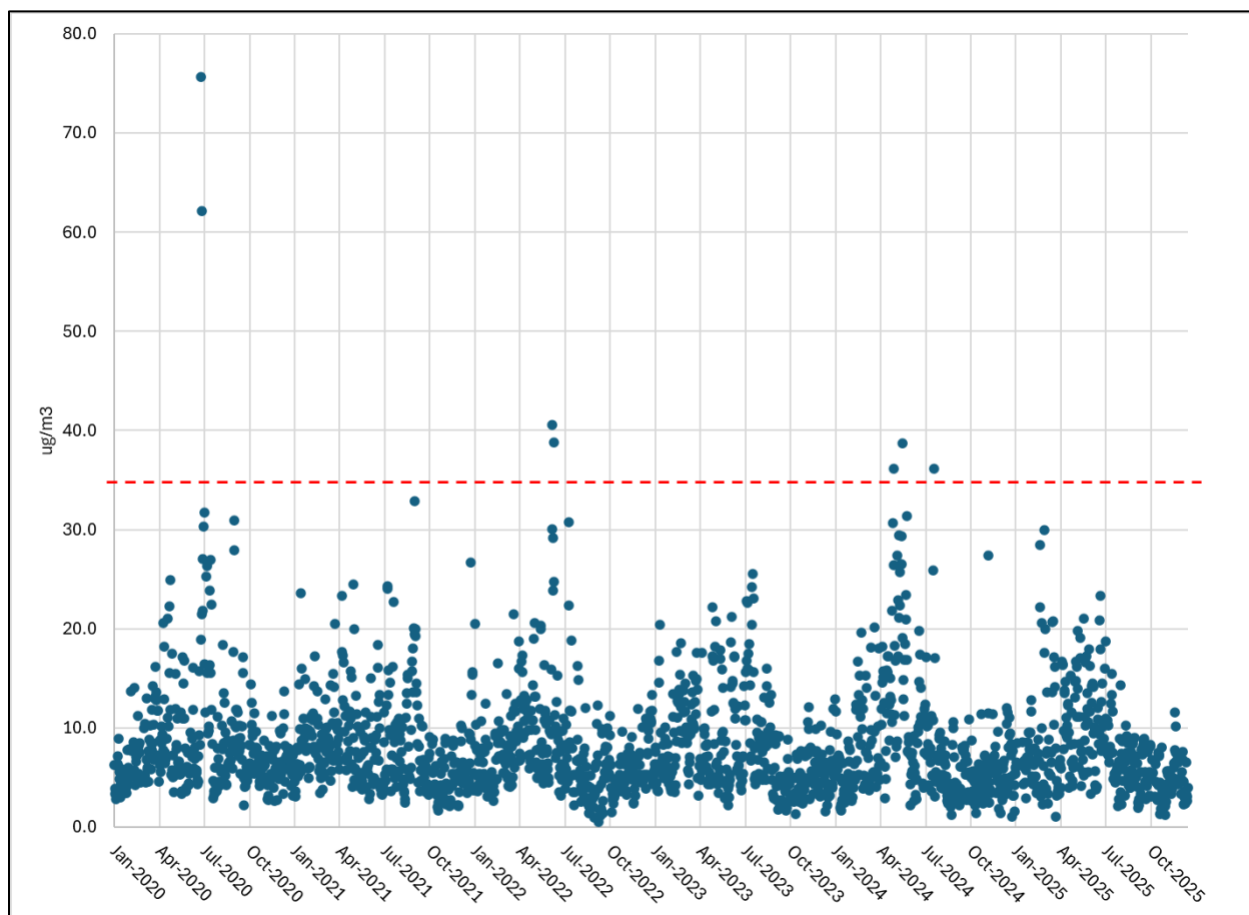
Figure 21. Mean 24-Hr PM 2.5 at PBway, Jan. 1, 2020 – Dec. 31, 2025, with NAAQS value 35 \mu\text{g}/\text{m}^3 (red dashed line).
