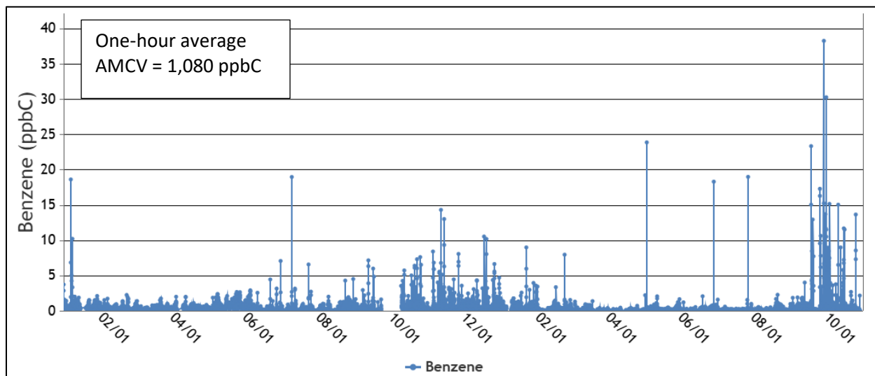
Figure 4. Hourly benzene concentrations at GF station, Jan. 1, 2024 – Oct. 31, 2025, ppbC units
