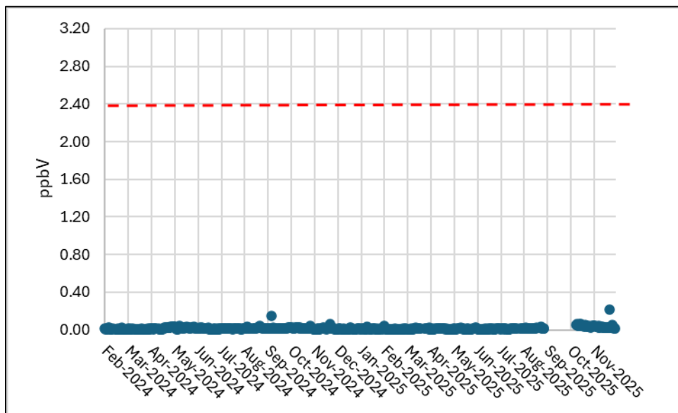
Figure 14. PBG AROMA EtO continuous analyzer 24-hour averages, Feb. 1, 2024 – Nov. 30, 2025, with TCEQ AMCV at 2.4 ppbV
