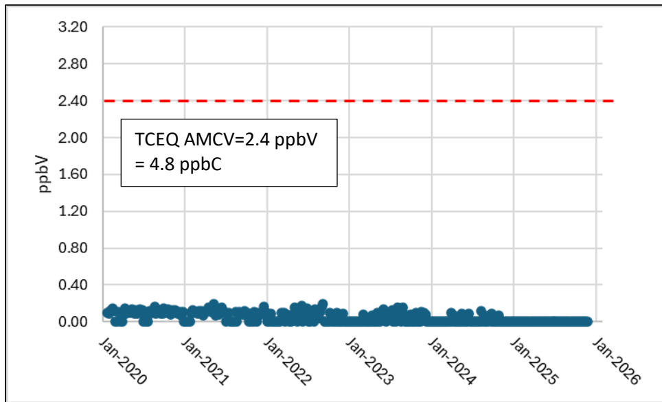
Figure 10. PBway EtO concentrations, every 6 th day samples Jan. 2020 through Nov. 2025, in comparison to TCEQ Air Monitoring Comparative Value
