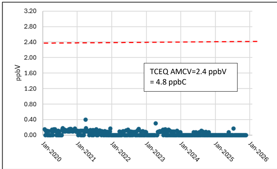
Figure 8. PBG EtO concentrations, every 6 th day samples Jan. 2020 through Nov. 2025, in comparison to TCEQ Air Monitoring Comparative Value
