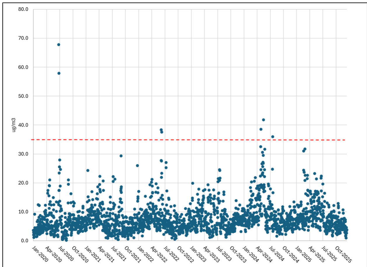
Figure 20. Mean 24-Hour PM2.5 at PBG, Jan. 1, 2020 – Dec. 31, 2025, with NAAQS scale 35µg/m³ (red dashed line).
