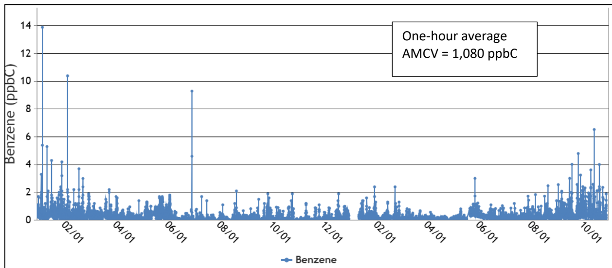
Figure 6. Hourly benzene concentrations at PBway station, Jan. 1, 2024 – Oct 31, 2025, ppbC units
