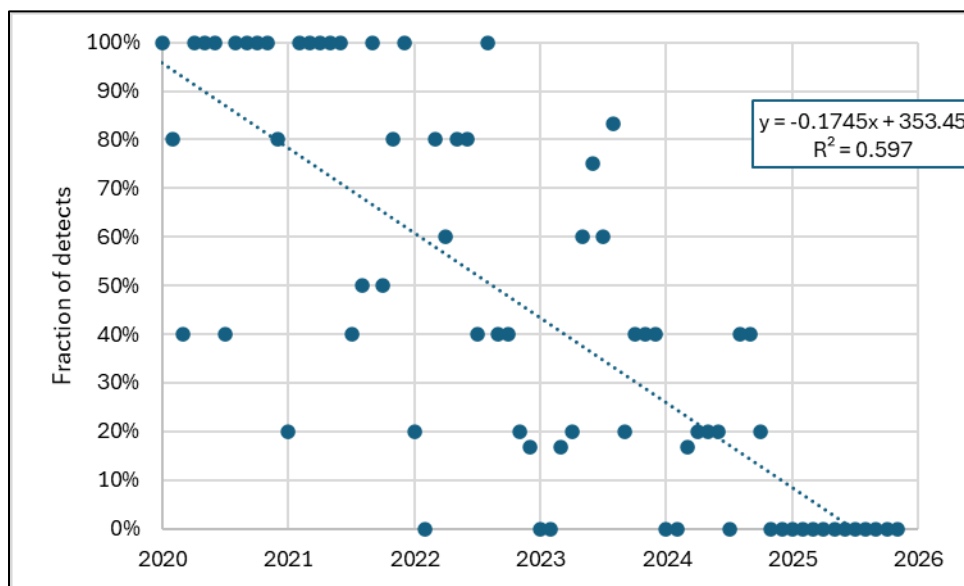
Figure 12. PBway percent of detections by sample each month, Jan. 2020 to Nov. 2025
